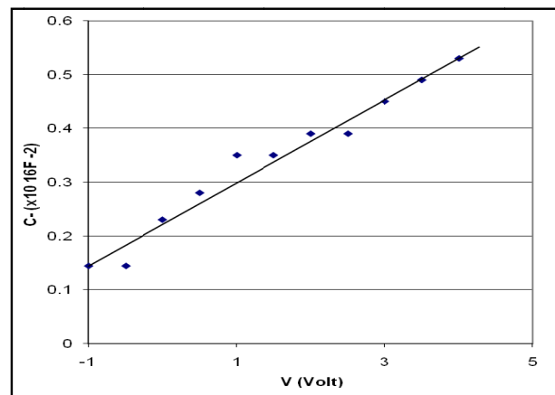
Fig. 2 C^{-2} -V plots for d_i = 18 nm
