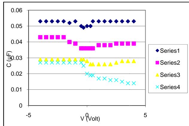
Fig. 1 C-V plots for d_i = 18 nm, 0.3 kHz [Series 1], 1 kHz [Series 2], 10 kHz [Series 3], and 50 kHz [Series 4]
