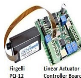
Fig. 4 Firgelli PQ-12 linear actuator and controller board
