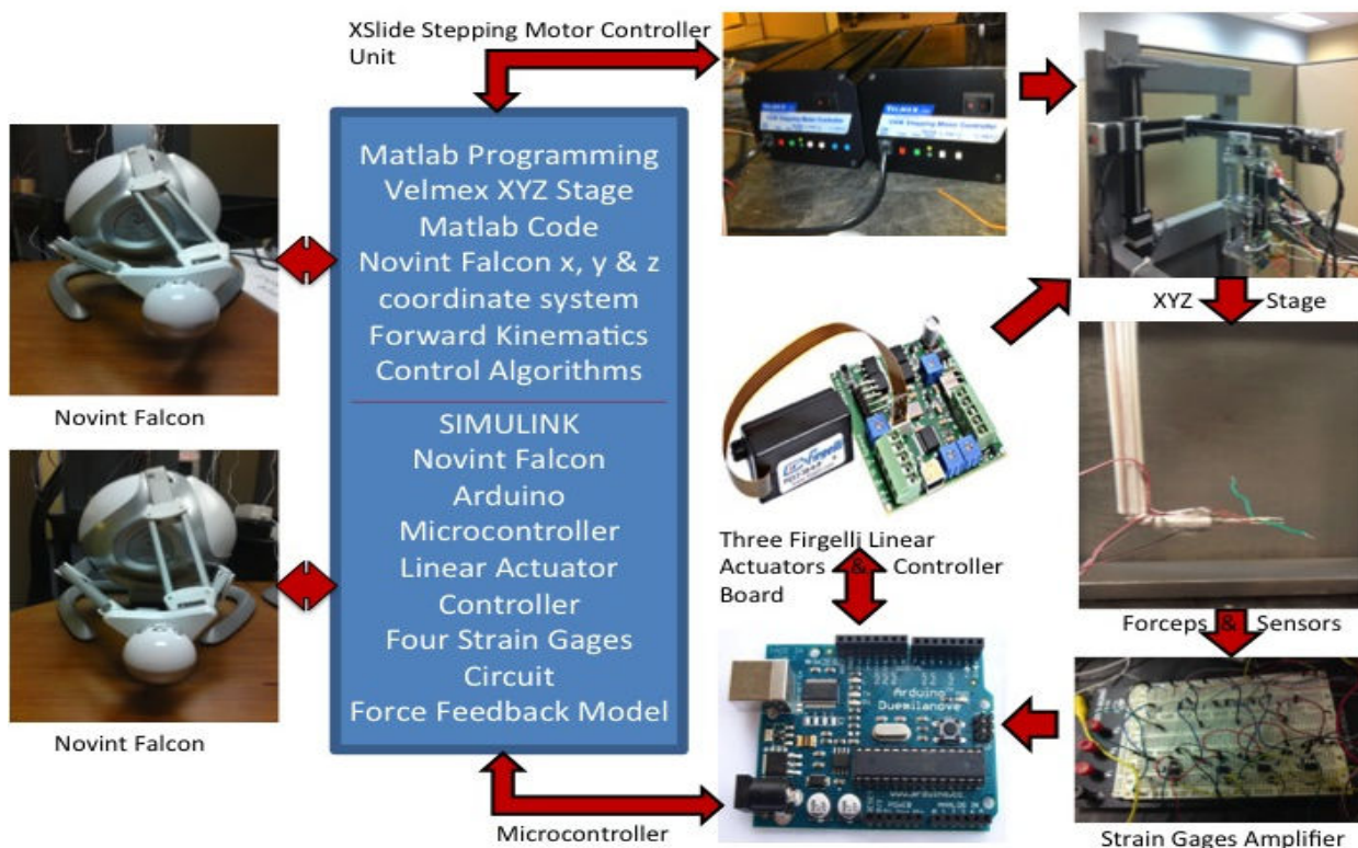
Fig. 5 Experimental setup for haptic feedback mechanism in real time
