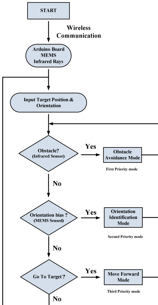
Fig. 4 Hybrid control mode for autonomous mobile robot
