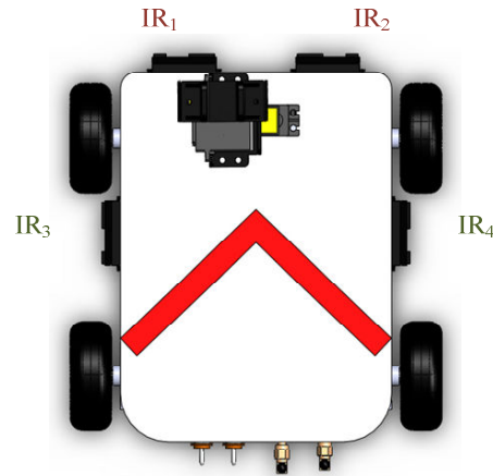
Fig. 5 IR sensors location on the AMR
