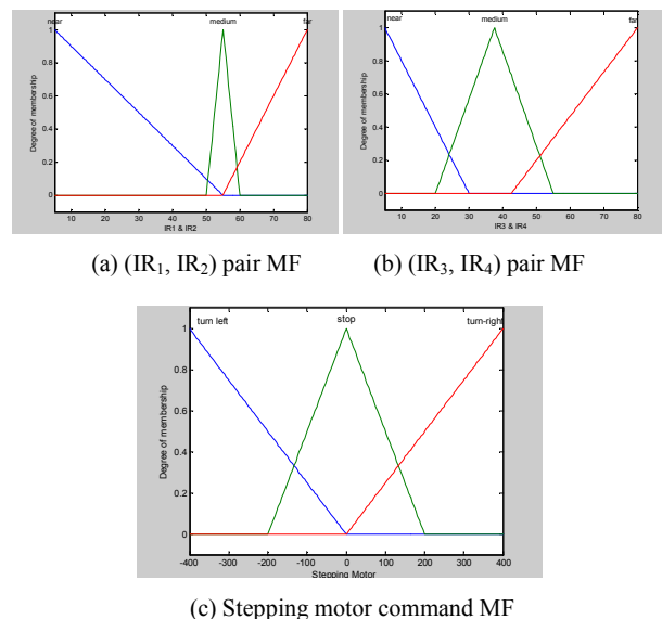
Fig. 6 Type I fuzzy controller for obstacle avoidance mode
