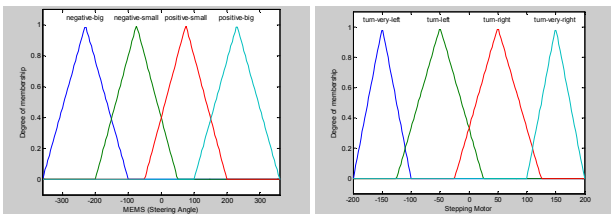
(a) MEMS sensor MF (b) Stepping motor MF
