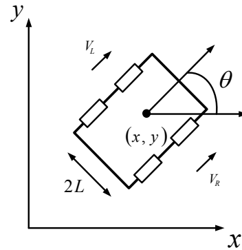
Fig. 1 Kinematic model of a mobile robot
