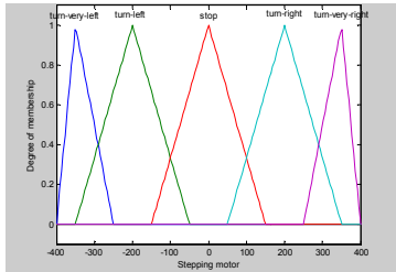
(c) Stepping motor command MFs
