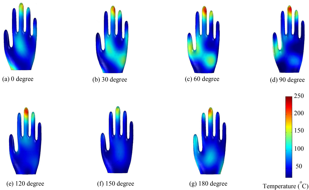
Fig. 7 The temperature distribution in NRG during microwave heating based on P = 100\text{ W} and t = 180\text{ s} at various rotation angle of NRG
