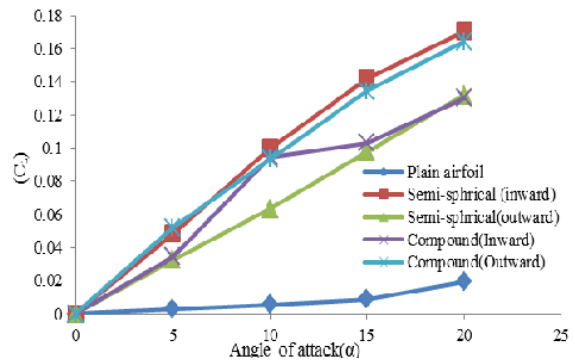
Fig. 7 Variation of C_L value of different dimple configuration
