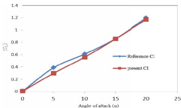
Fig. 2 Comparison between reference and present computational value
