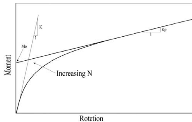
Fig. 2 Parameters of Richard model
