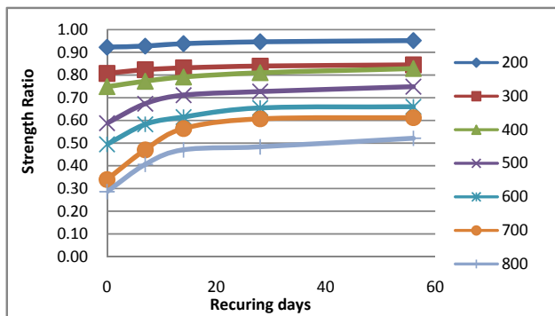
Fig. 3 Strength improvement through recuring for concrete subjected to heating for 2 hrs
