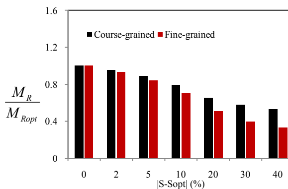
Fig. 1 Effect of moisture on the resilient modulus
