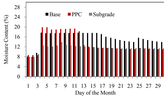
Fig. 6 Moisture variations in a month (July, 2012)
