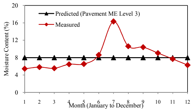
Fig. 11 Measured and predicted moisture data in subbase layer
