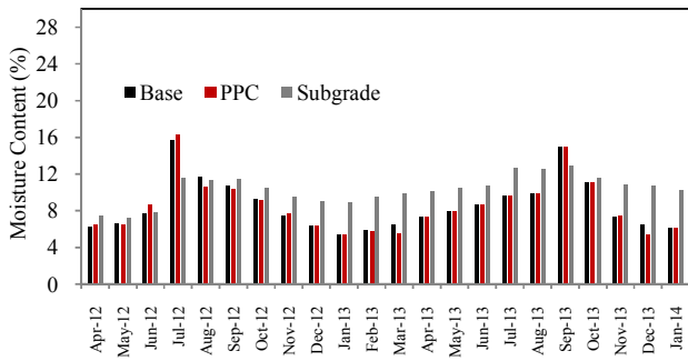
Fig. 8 Moisture variations from 2012 to 2014)
