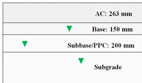
Fig. 2 Elevations of the installed moisture probes
