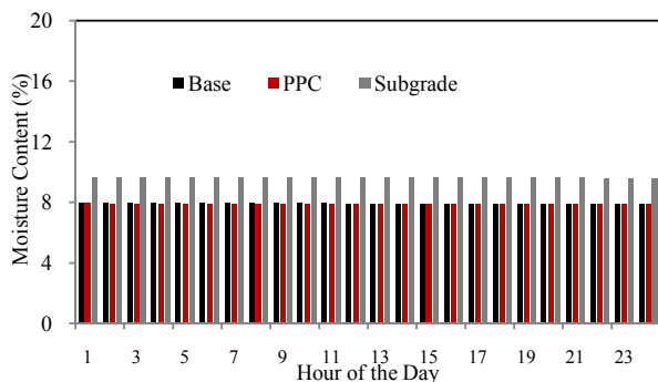
Fig. 4 Moisture variations in subgrade on October 1, 2012
