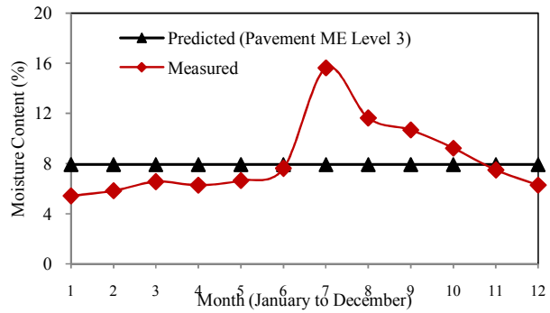
Fig. 10 Measured and predicted moisture data in base layer
