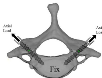
Fig. 5 Axial load act on top of bone screw
