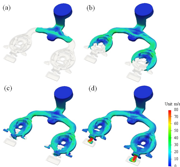
Fig. 5 Sequential images of melted aluminum flowing into the mold cavity at (a) t = 0.015 sec, (b) t = 0.021 sec, (c) t = 0.024 sec and (d) t = 0.025 sec
