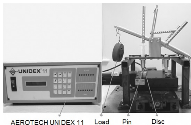
Fig. 1 Pin-on-disc (AEROTECH UNIDEX 11)
