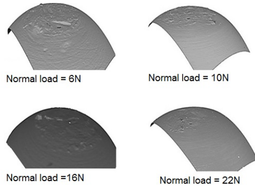
Fig. 12 Pin wear scar measured by using alicona
