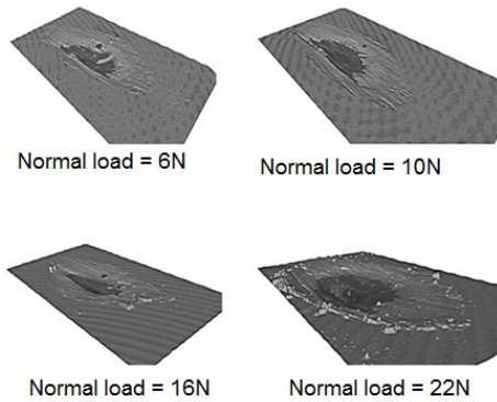
Fig. 11 Disc wear scar measured using alicona
