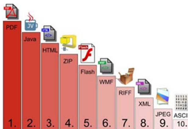
Fig. 1 AVTEST Report
