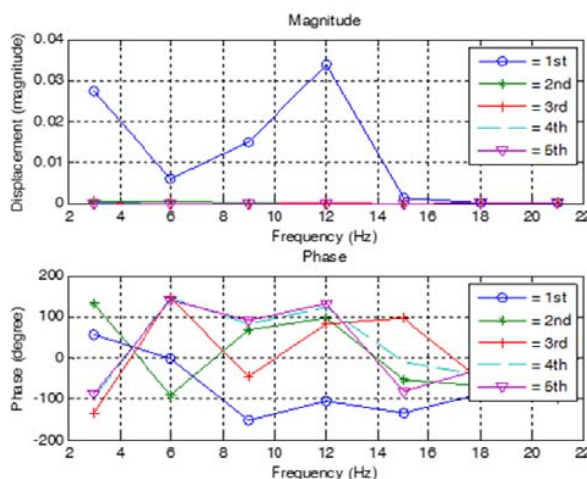
Fig. 20 Magnitude displacement and phase angle for 1000 V at varies frequency
