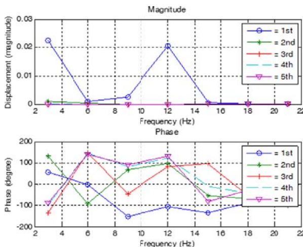
Fig. 19 Magnitude displacement and phase angle for 500 V at varies frequency
