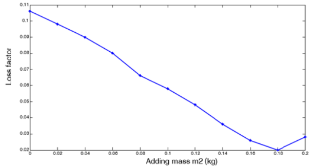
Fig. 8 Loss factor – Mass
