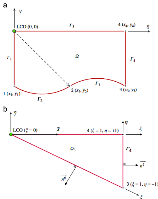
Fig. 2 Modeling of 2D bounded domain, and the LCO: (a) in global coordinates system, and (b) in scaled boundary local system
