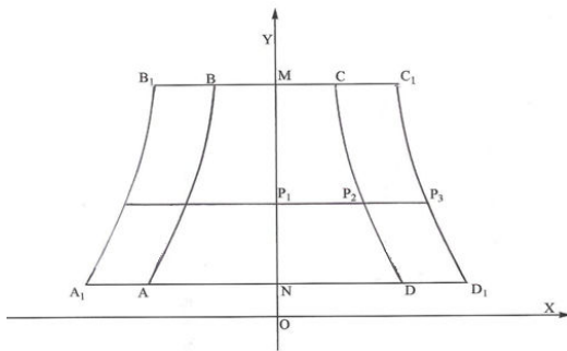
Fig. 1 Scheme of graded stretching of trapezoidal sample. Explanations are given in the text
