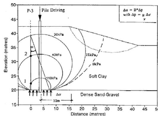
Fig. 1 Pore water pressure changes due to pile driving [4]
