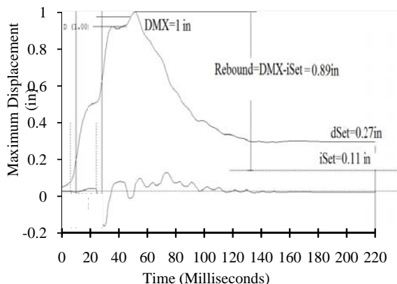
Fig. 2 Typical PDA pile top displacement versus time diagram from one hammer blow for FDOT HPR site
