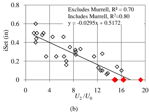
Fig. 7 Correlation includes [9] between Rebound, Permanent-set and (a) CPTu pore water pressure, and (b) ratio of CPTu pore water pressure and hydrostatic pressure ( u_0 )
