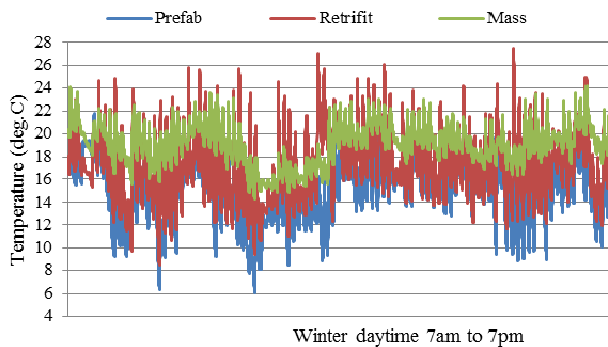
Fig. 6 Indoor air temperatures during the winter daytime
