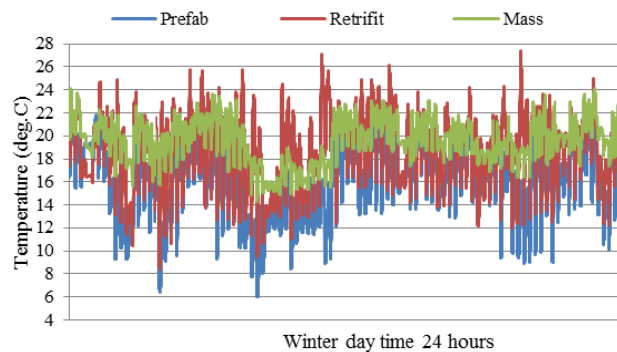
Fig. 4 Indoor air temperatures during the winter months
