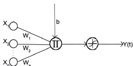
Fig. 1 Single Neuron as a classifier
