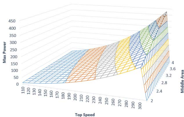
Fig. 2 Required Peak Motor Power
