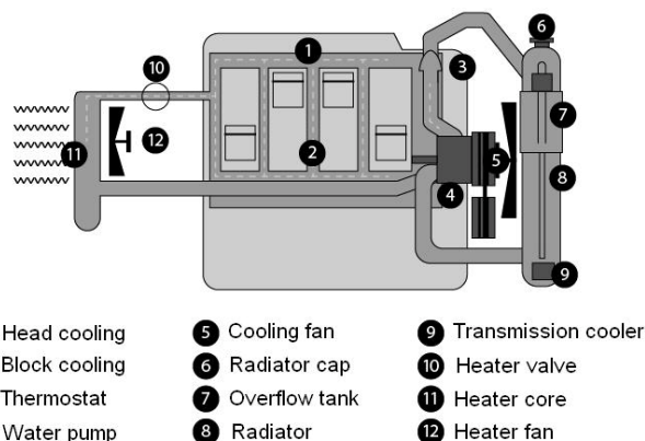
Fig. 1 Cooling System
