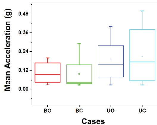
Fig. 7 Spread of mean of accelerations of all the subjects for all the cases (BO, BC, UO and UC) obtained from accelerometer
