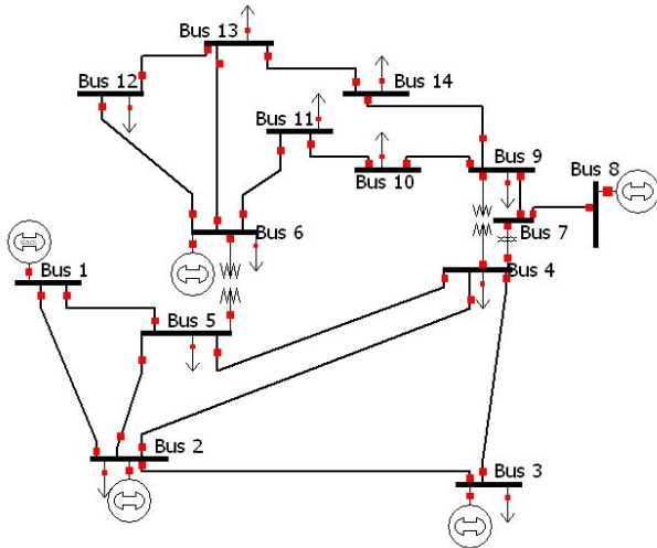
Fig. 3 IEEE 14 bus test network
