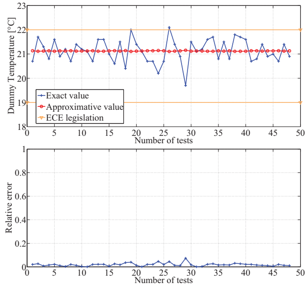
Fig. 7: Estimation's curves for the dummy temperature
