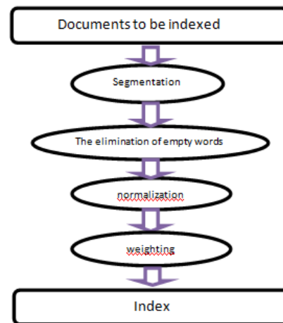
Fig. 2 Phases of automatic indexation
