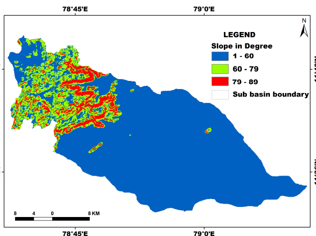
Fig. 4 Slope map
