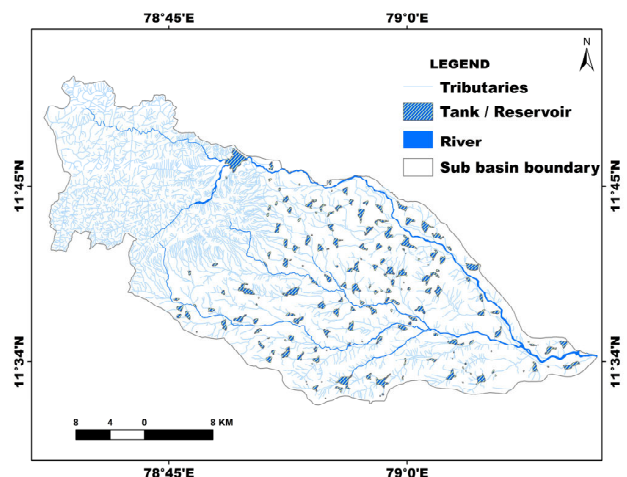
Fig. 3 Drainage map
