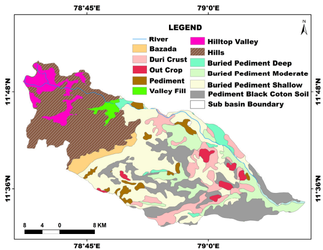
Fig. 7 Geomorphology map
