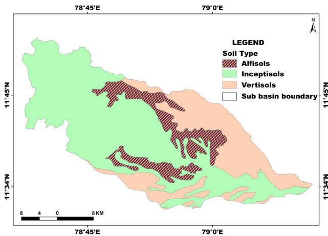
Fig. 6 Soil map
