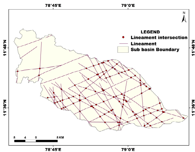
Fig. 8 Lineament map
