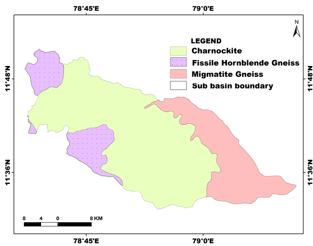
Fig. 5 Geology map
