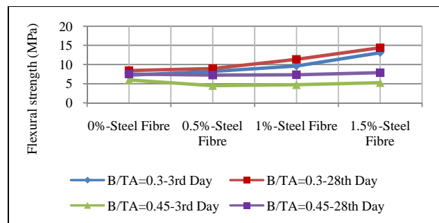
Fig. 2 Flexural strength property of steel fibre reinforced geopolymer concrete
