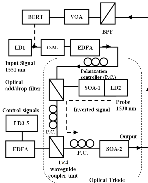
Fig. 3 Experimental setup
