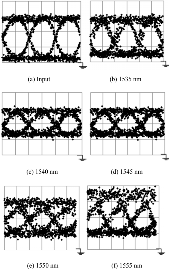
Fig. 4 Eye diagrams of input and output signals (50μW/div, 50ps/div)
