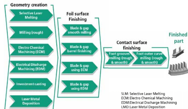
Fig. 6 Examination of potential manufacturing process chains
