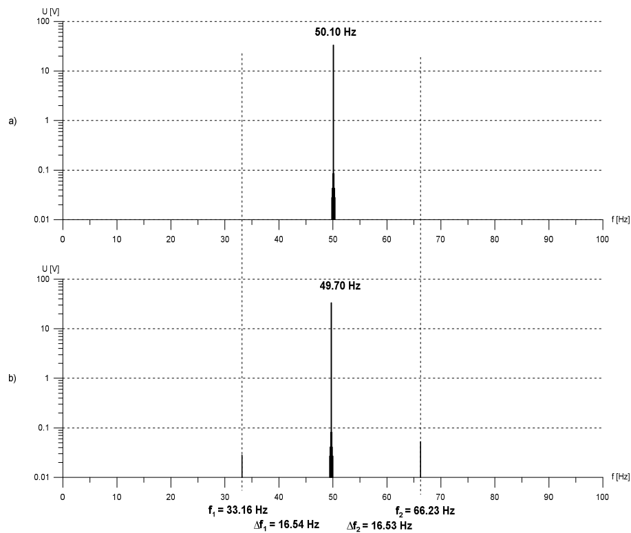
Fig. 8 Frequency spectra induced voltage of the generator - the results of the simulations
