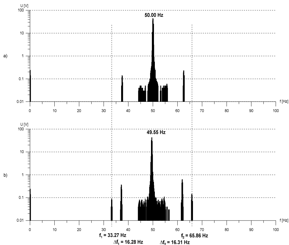
Fig. 9 Frequency spectra induced voltage of the generator - the results of the real measure
