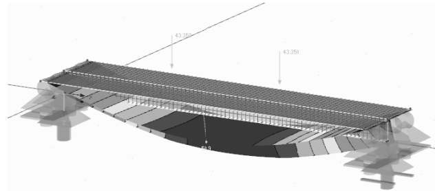
Fig. 2 Results of numerical model of composite beam
