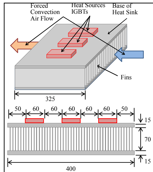
Fig. 1 Schematics of a conventional heat sink
