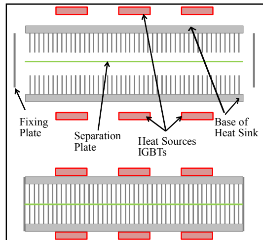
Fig. 2 Schematics of a symmetrically arranged heat sink
