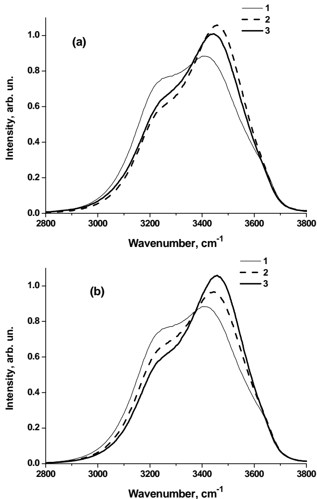
Fig. 2 Valence Raman bands of water. (a): 1 – distilled water; 2 – \text{CsI} , 2 M; 3 – \text{NaCl} , \text{NH}_4\text{Br} , \text{Li}_2\text{SO}_4 – 0.4 M, \text{KNO}_3 и \text{CsI} – 0.6 M. (b): 1 – distilled water; 2 – \text{CsI} , 1 M; 3 – \text{CsI} , 2 M.
