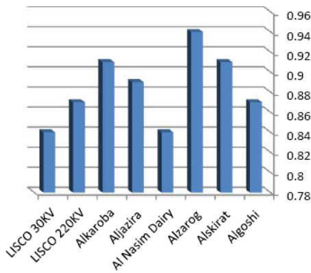
Fig. 7 Power Factor comparison
