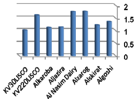
Fig. 8 K-Factor Comparison
