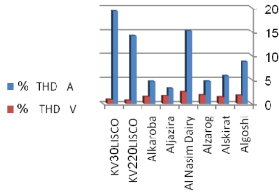
Fig. 9 THD Factor for the voltage and the current
