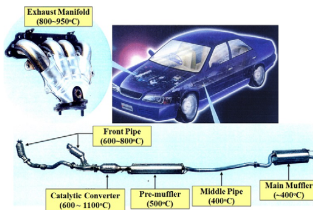
Fig. 1 Automotive exhaust system components
