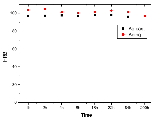
Fig. 8 Hardness measured after exposition at 1200°C for various time intervals
