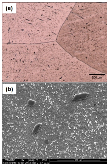
Fig. 10 Optical micrograph (a) and SEM image (b) showing carbides precipitated during hot exposition at 1200°C for 200 hrs
