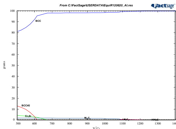
Fig. 4 Calculated phase equilibrium showing stable phases and their weight fractions of Fe-20Cr-5Al stainless steel
