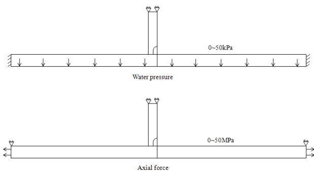
Fig. 4 Loading condition
