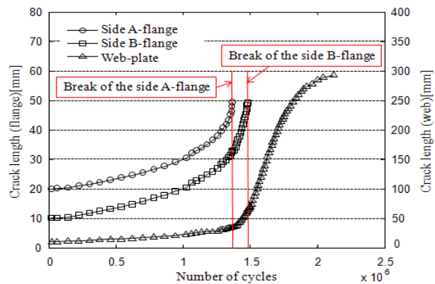
Fig. 9 Simulated crack growth lives in the flange and the web-plate under water pressure loading
