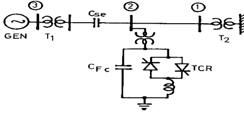
Fig. 1 Study system: IEEE FBM [16]
