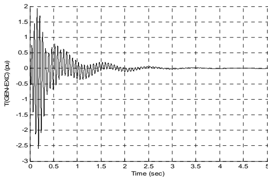
Fig. 7 Variation of shaft torsional torque (GEN-EXC)with CBVLC
