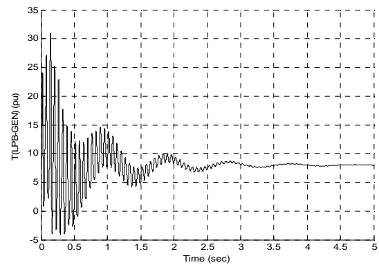
Fig. 6 Variation of shaft torsional torque (LPB-GEN)with CBVLC
