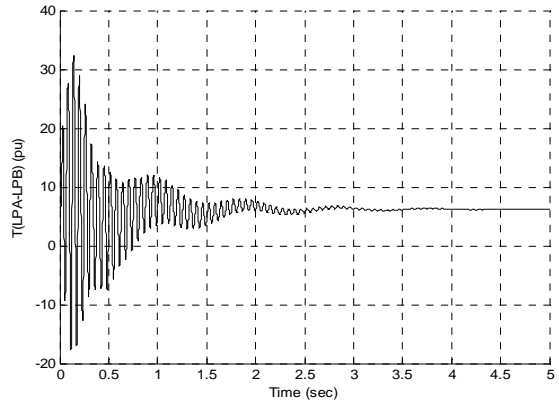
Fig. 5 Variation of shaft torsional torque (LPA-LPB)with CBVLC
