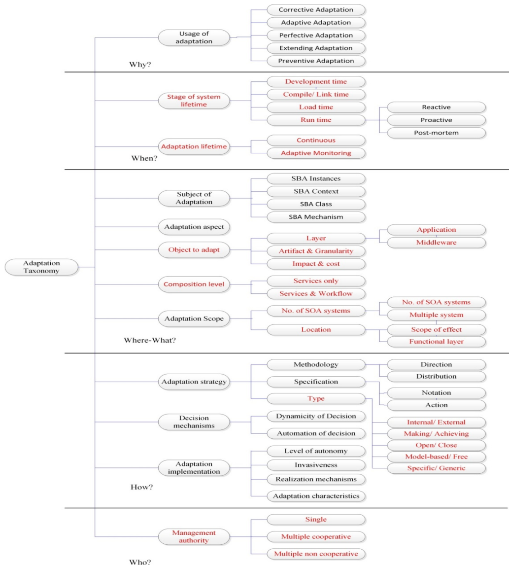
Fig. 1 Adaptation taxonomy
