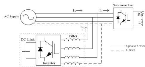
(a) 3-phase 3-wire and 3-phase 4-wire topology
