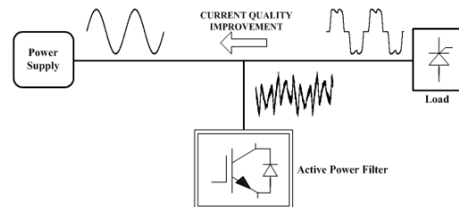
Fig. 1 Fundamental representation of APF
