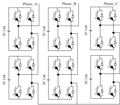
(c) 3-phase 3-wire with multilevel topology
