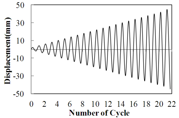
Fig. 4 Loading protocol
