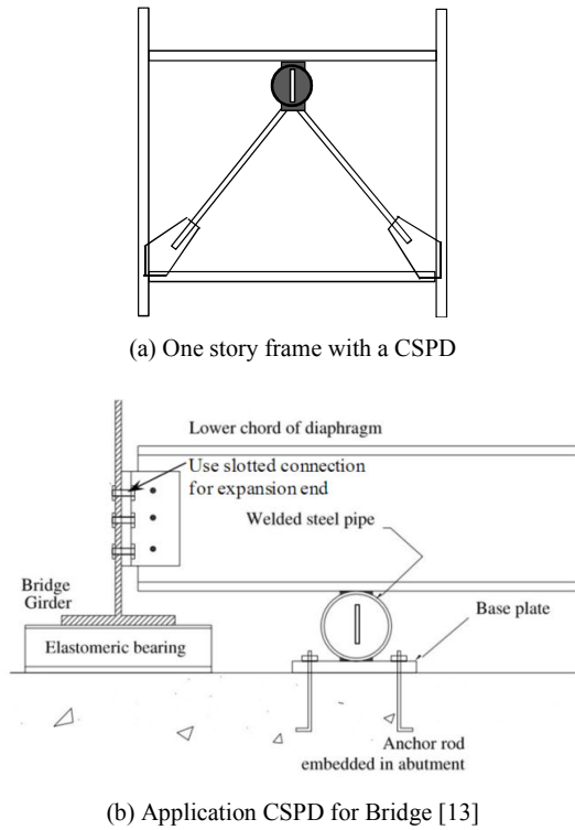
Fig. 1 Samples of circular shear panel damper incorporated into structures
