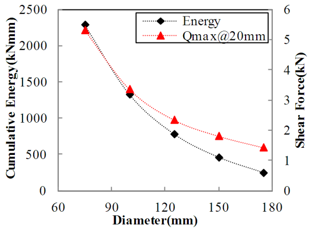
Fig. 13 Cumulative energy and shear capacity of CSR
