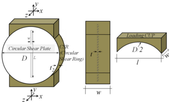
Fig. 2 Specimen Detail
