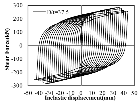
Fig. 6 Shear force-Inelastic rotation relationship
