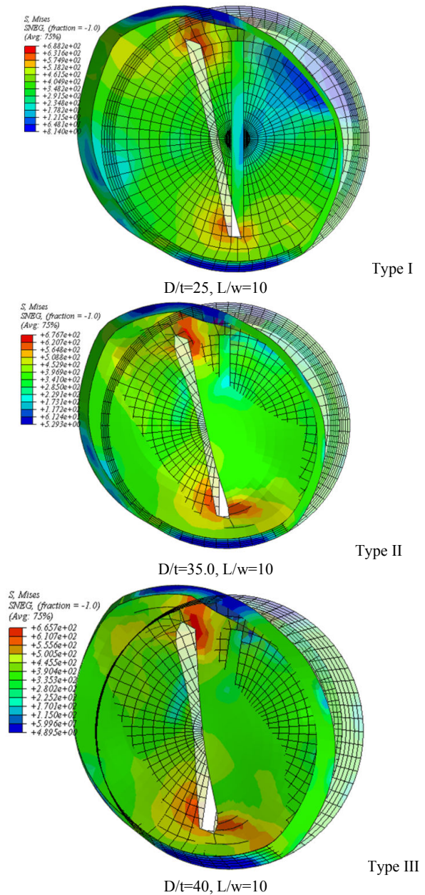
Fig. 9 Deformation mode and von Mises stress distribution
