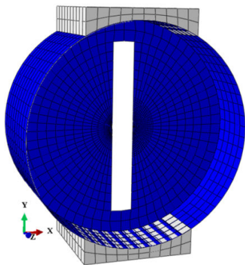
Fig. 3 3D analysis model
