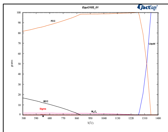
Fig. 4 Calculated phase equilibrium showing stable phases and their weight fractions of 310S stainless steel
