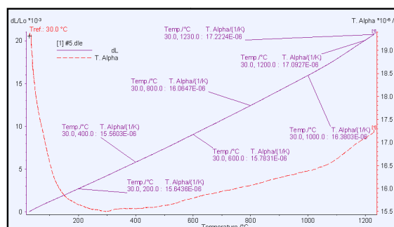
Fig. 3 Dilatation and CTE measured on as-cast 310S stainless steel ingot at temperatures ranging from room temperature to 1200°C
