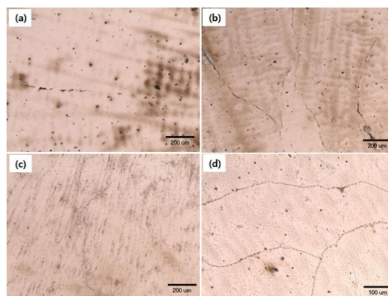
Fig. 8 Microstructure observed after tensile tests conducted at temperatures of 1200°C (a), 1100°C (b), 1000°C (c), and 900°C (d), respectively
