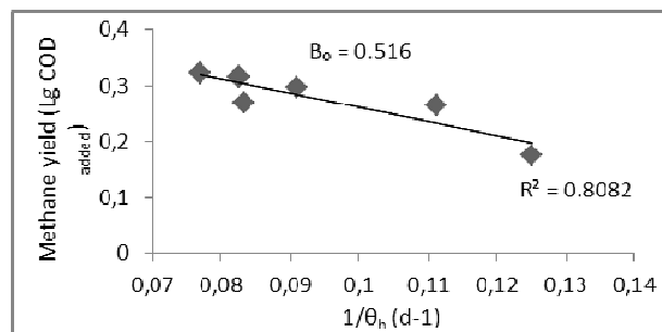
Fig. 2 Determination of ultimate methane yield ( B_0 )
