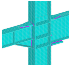
(c) One sided haunch connection (Y=3)
