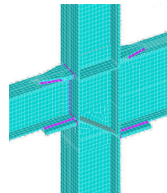
(a) Inclined continuity plate (Y=1)
