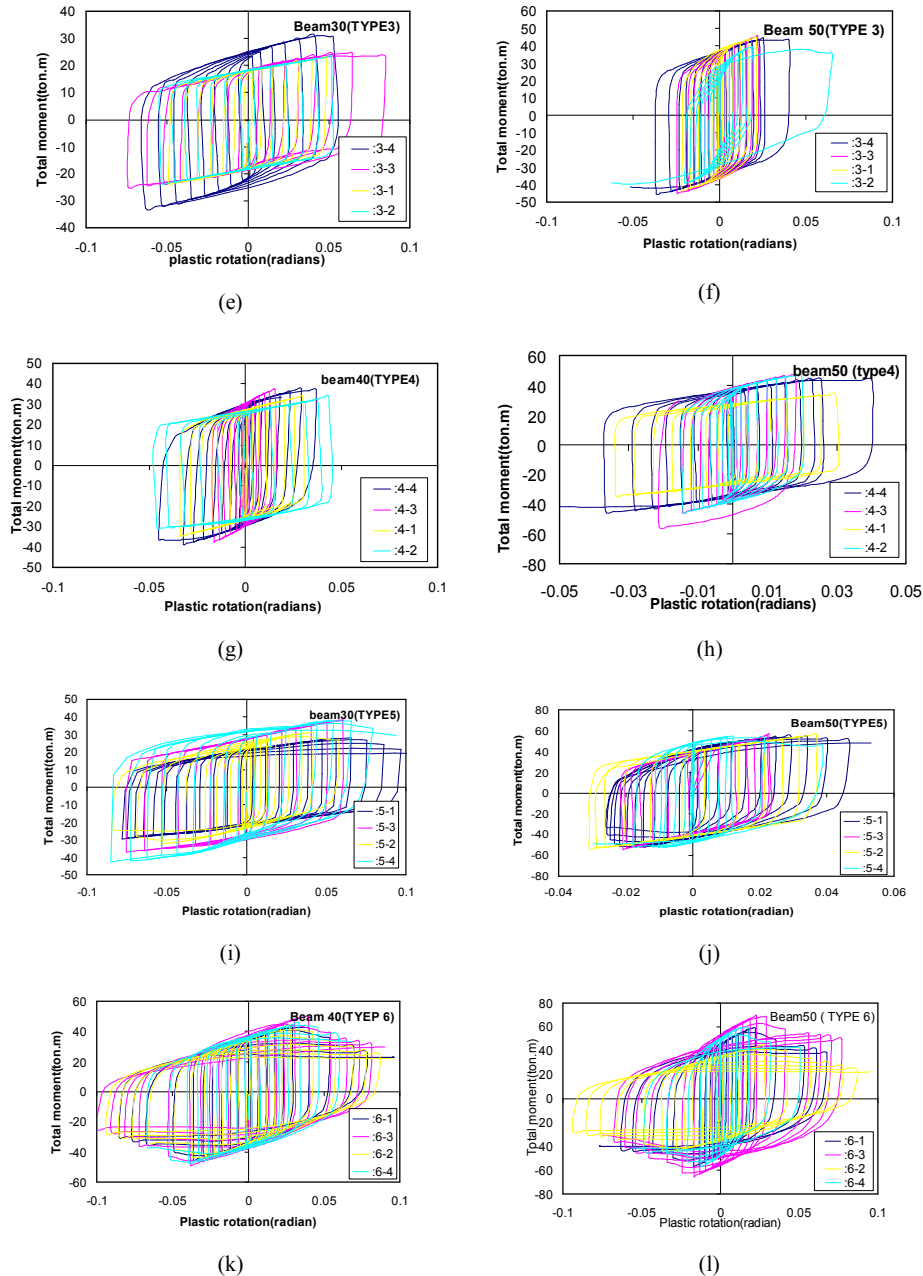
Fig. 4 Cyclic response of analytical models
