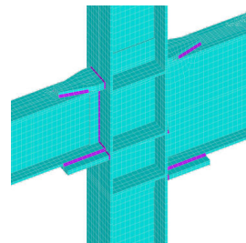
(b) Straight continuity plate (Y=2)
