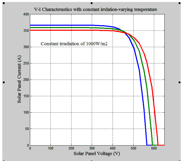
Fig. 4 Simulink model of solar panel (810 strings) I-V Characteristic curves at different cells working temperature (HIP-180BA3, Tc =25°C, 50°C, 75°C)
