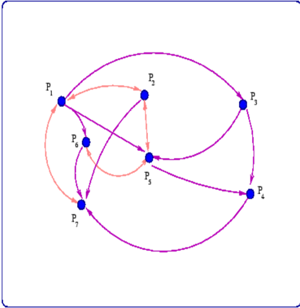
Fig. 3 (b) Graph representation
