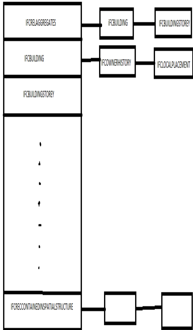
Fig. 3 (a) Data Structure List Representation
