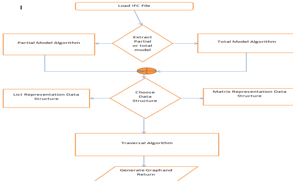
Fig. 2 Flowchart for selecting traversal algorithm
