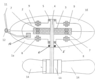
Fig. 10 Design of mobile micro HPP (section view along the rotation axis)
