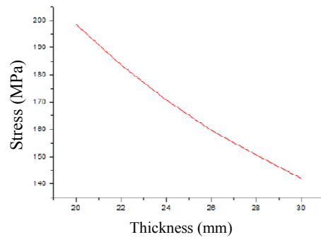
Fig. 9 Von Mises stress function in thickness
