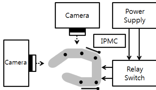
Fig. 2 Experimental setup for pinching motion analysis
