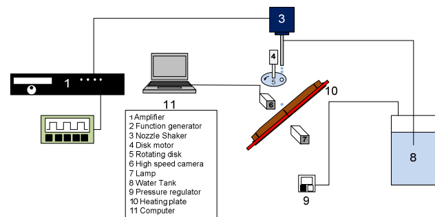
Fig. 2 Experimental Apparatus
