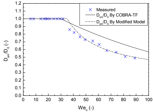
Fig. 9 Modified Model
