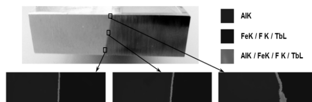
Fig. 6 Elemental Composition of Bimetallic FSW Joint
