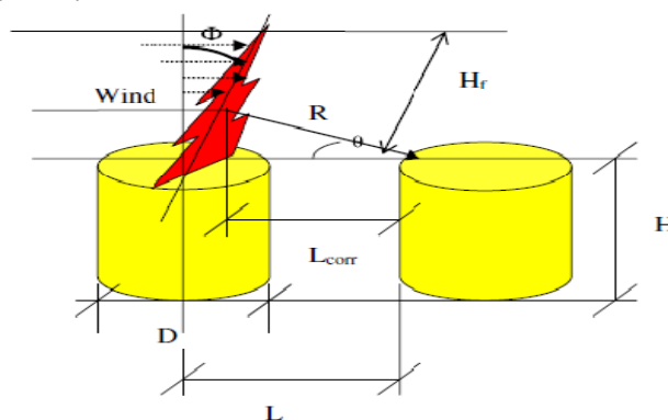
Fig. 3 Schematic diagrams for tank on fire under cross-wind condition [11]
