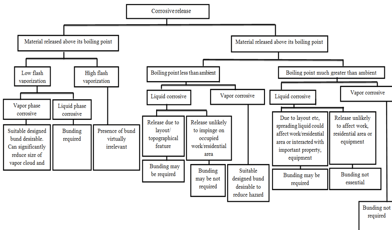
Fig. 1 Decision trees for the design of bunds for a) flammable, b) toxic and c) corrosive material
